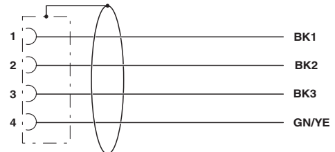
Contact assignment of the M12 socket
